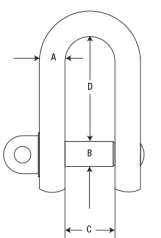
Screw Pin Dee Shackle
